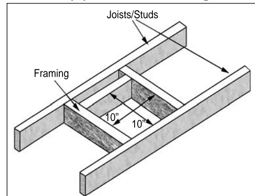
Figure 23. Vent Framing For Wall or Ceiling.
