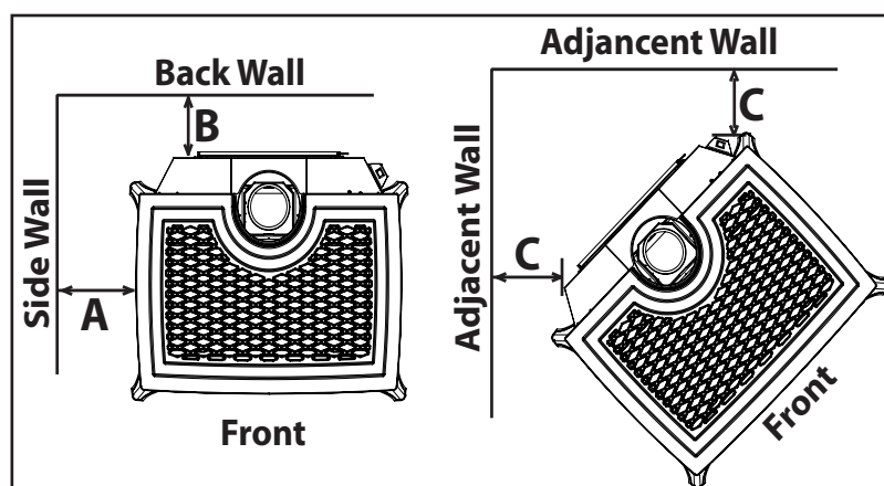
Figure 21: Clearance to Combustibles
