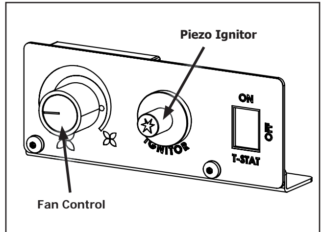
Figure 6. Control Panel
