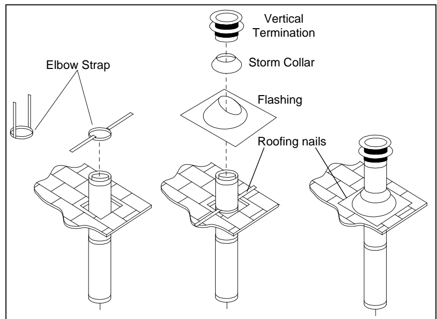
Figure 30. Vertical Vent Termination
