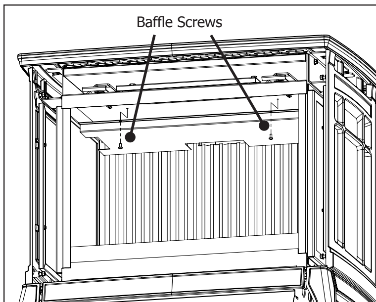
Figure 27: Baffle Removal
